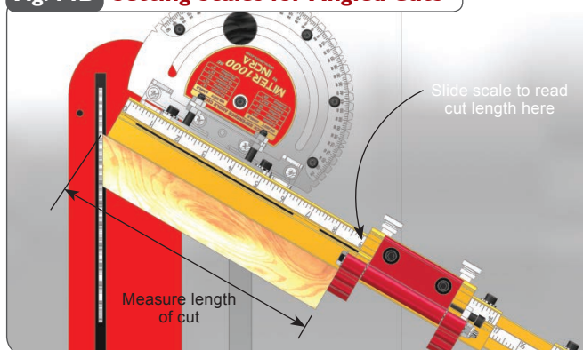
Fig. 15 Micro Adjusting
