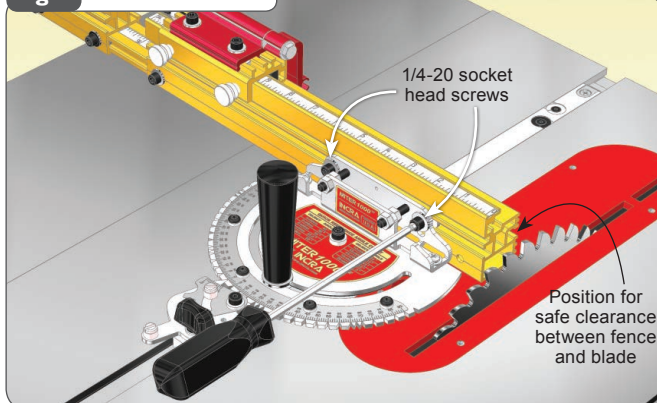
Fig. 5 Attach Fence
