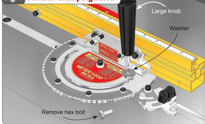
Fig. 2 Attach T-Clip
